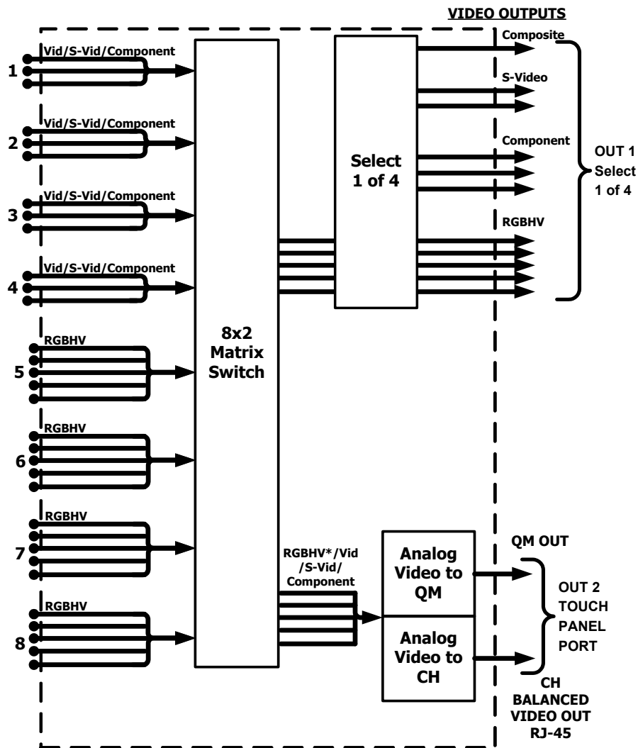
Video Block Diagram of the MPS-200
