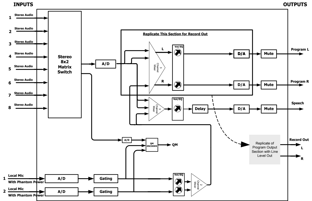
Audio Block Diagram of the MPS-200
