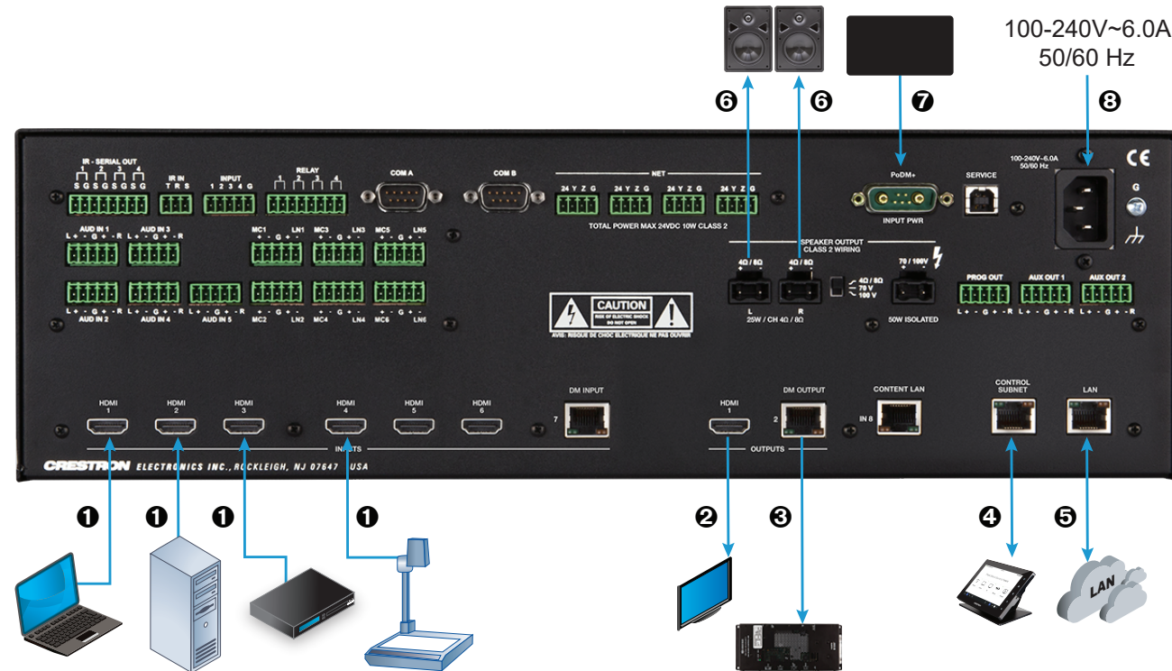
DMPS3-4K-250-C-AIRMEDIA (Rear View)
