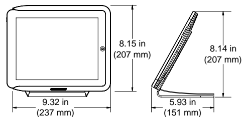
IDOC-PAD-DSC Dimensions
