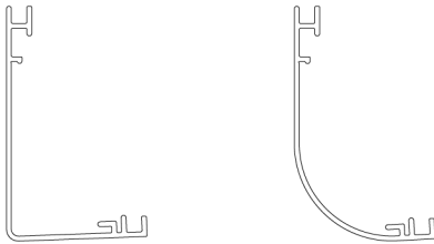
Square and Round Fascias: CSA-ARCH3-BRKT-DUAL
