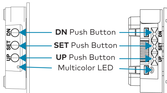
Crestron CSM-QMTDC Motor Multicolor LED and Push Button Orientation
