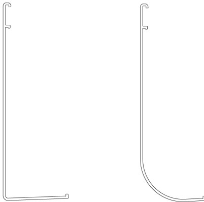
Square and Round Fascias: CSA-ARCH3-BRKT-DUAL
