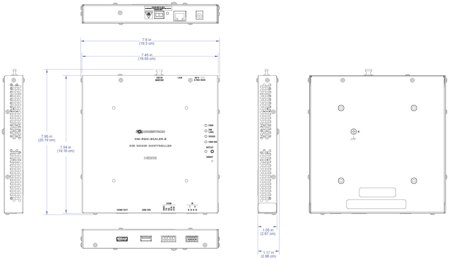
UNIT WITHOUT BRACKET INSTALLED
