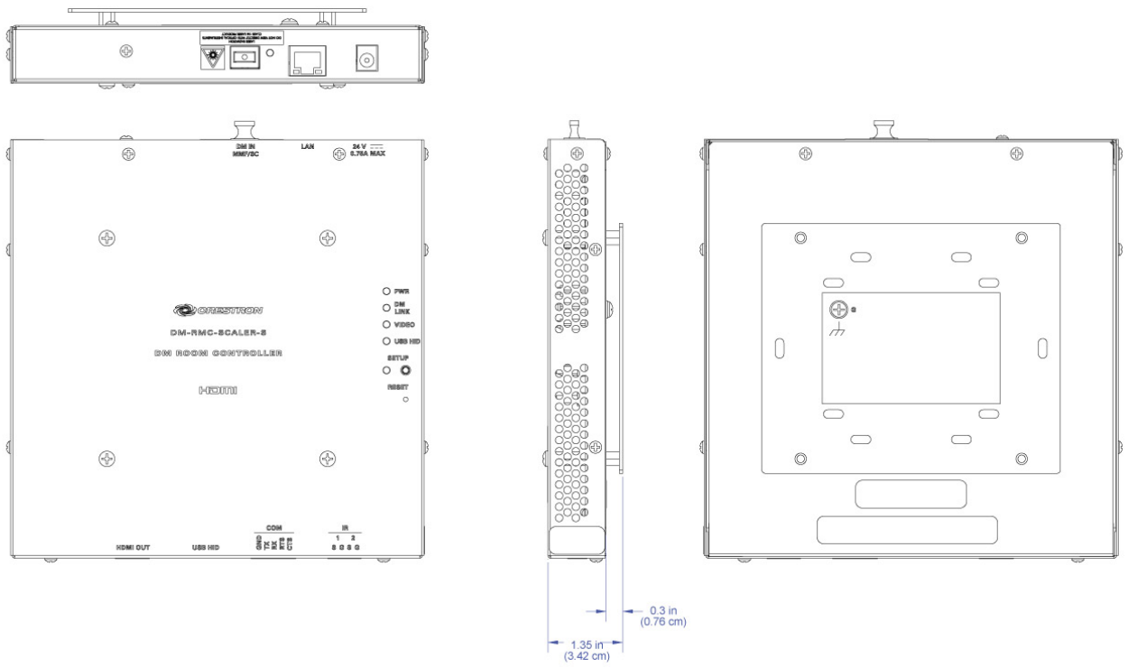
UNIT WITH BRACKET INSTALLED
