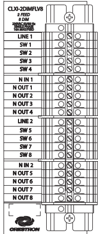
CLTI-2DIMFLV8 Terminal Block with Left-Side CLXI-2DIMFLV8 Label
