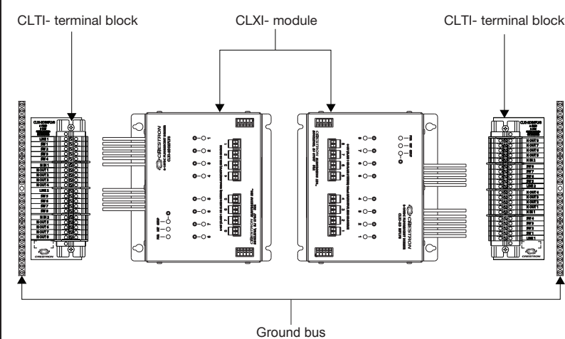
Terminal Block and Module Layout for a Double-Wide Enclosure (CLTI-2DIMFLV8 and CLXI-2DIMFLV8 Shown)
