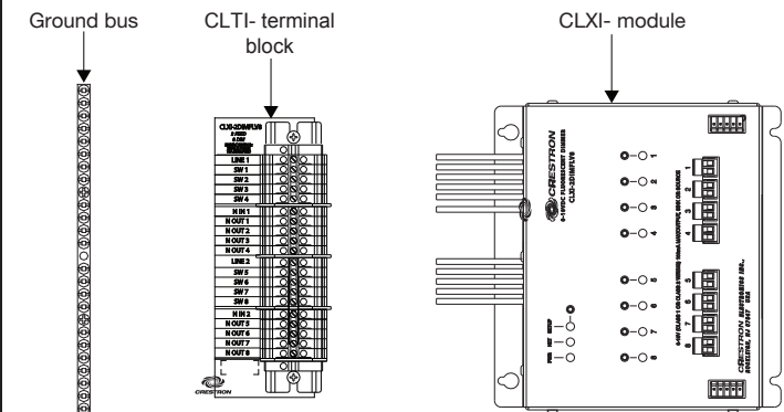
Terminal Block and Module Layout for a Double-Wide Enclosure (CLTI-2DIMFLV8 and CLXI-2DIMFLV8 Shown)
