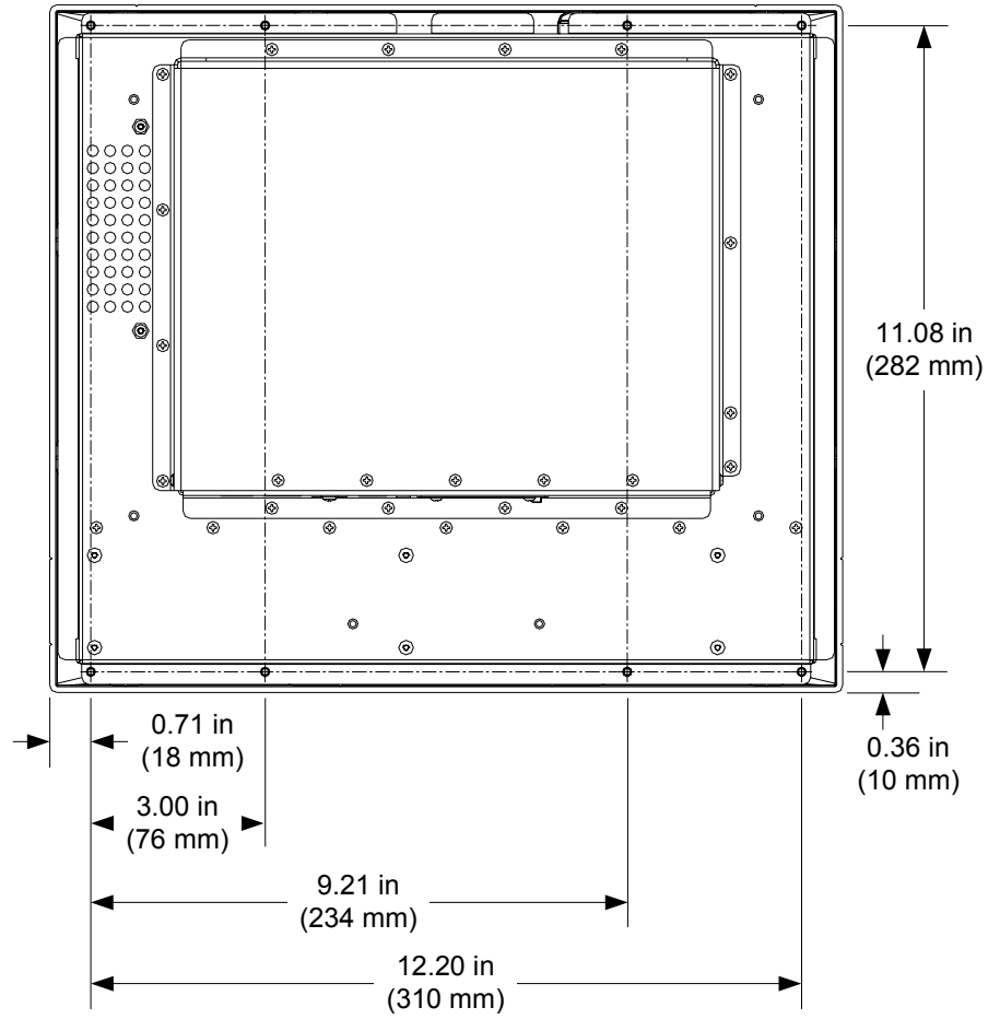
TPMC-12L Overall Dimensions (Rear View)
