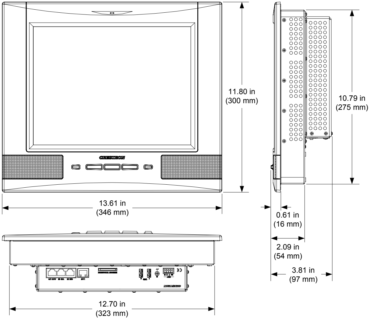
TPMC-12L Overall Dimensions (Front, Side and Bottom Views)
