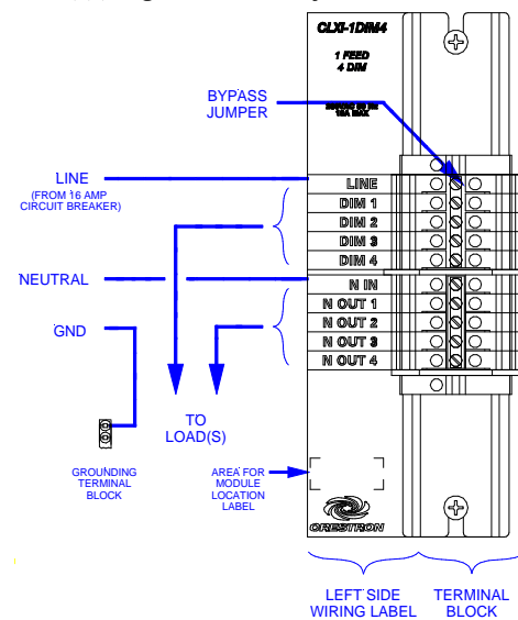
Wiring Diagram of the Terminal Block to the Feed and Load(s) (Right Side Double-wide Enclosures)
