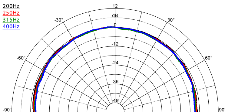
SAROS IC4T – Dispersion Pattern, 200 Hz - 400 Hz
