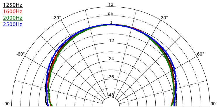
SAROS IC4T – Dispersion Pattern, 1250 Hz - 2500 Hz
