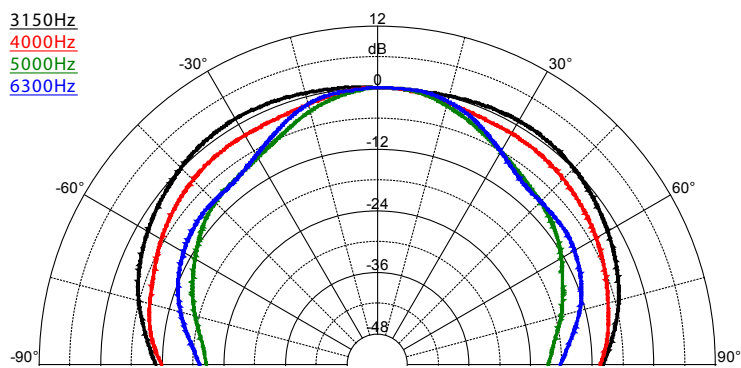
SAROS IC4T – Dispersion Pattern, 3150 Hz - 6300 Hz
