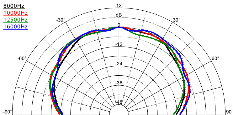
SAROS IC4T – Dispersion Pattern, 8000 Hz - 16000 Hz
