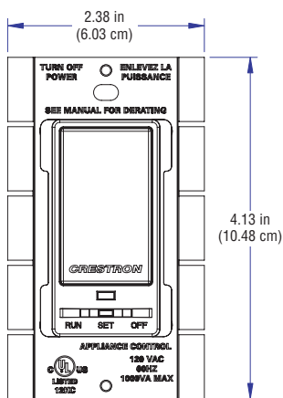
CLW-SW1RF and CLW-SWS1RF Front View
