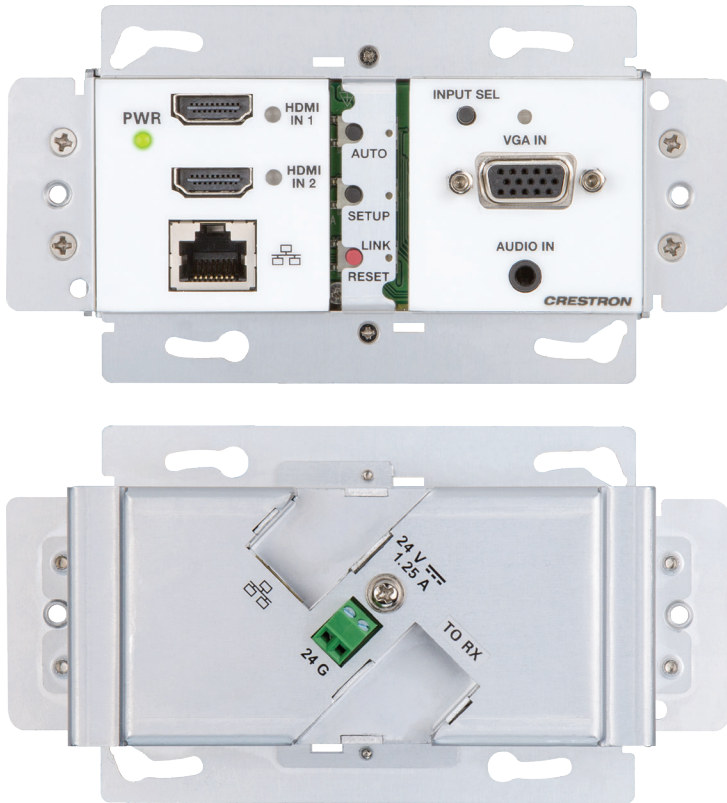
HDI-TX-301-C-2G-E Transmitter – Front & Rear Views White version shown with no faceplate
