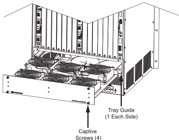
DM-MDA-64-FANTRAY Installation
