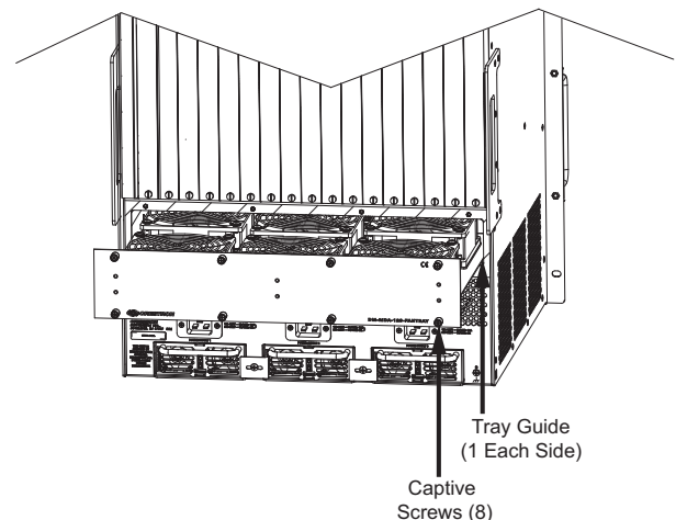
DM-MDA-128-FANTRAY Installation
