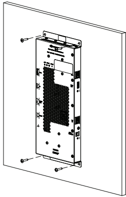
Mounting onto a Wall
