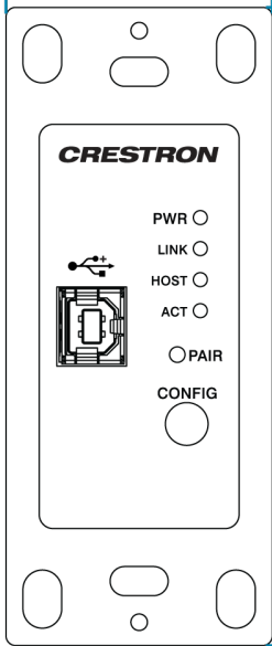
DM-NUX-L2-1G
