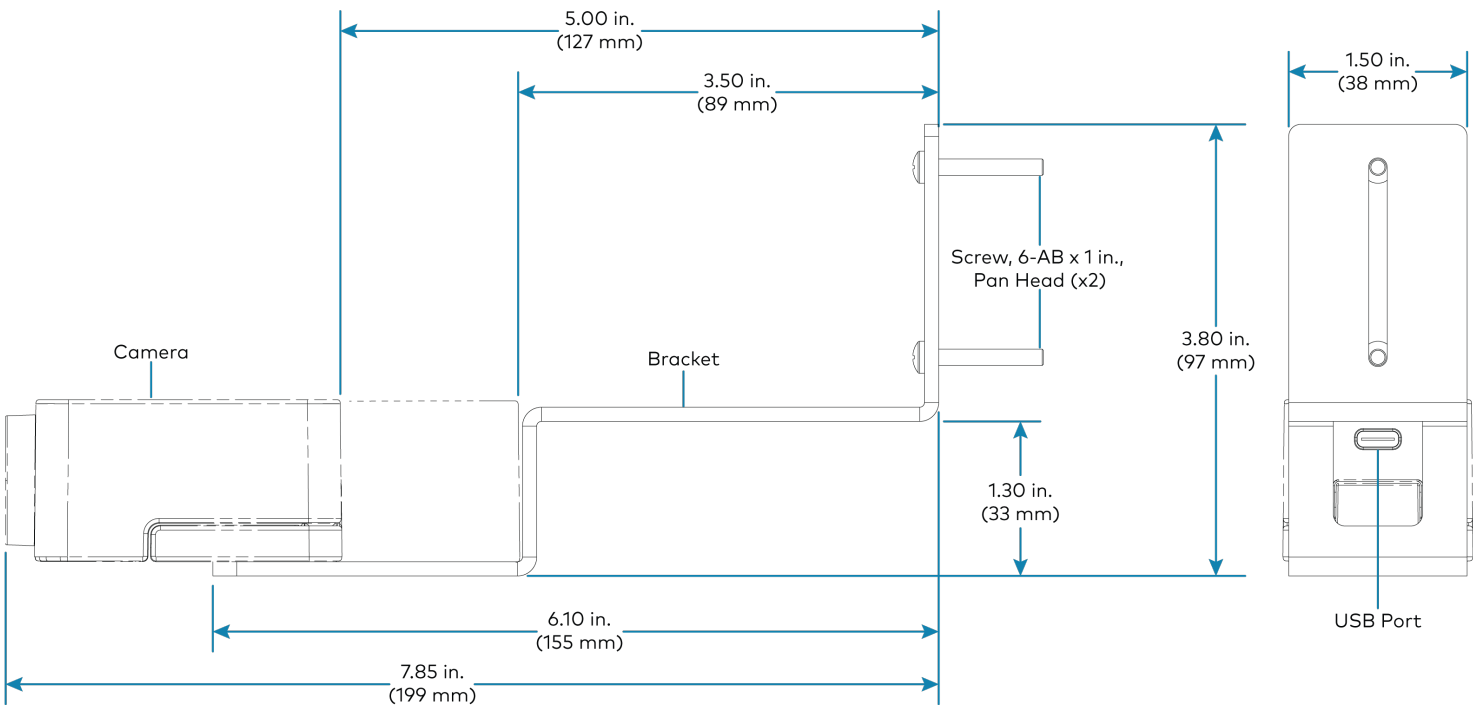
Large Bracket (CCS-CAM-USB-F-400 camera shown)
