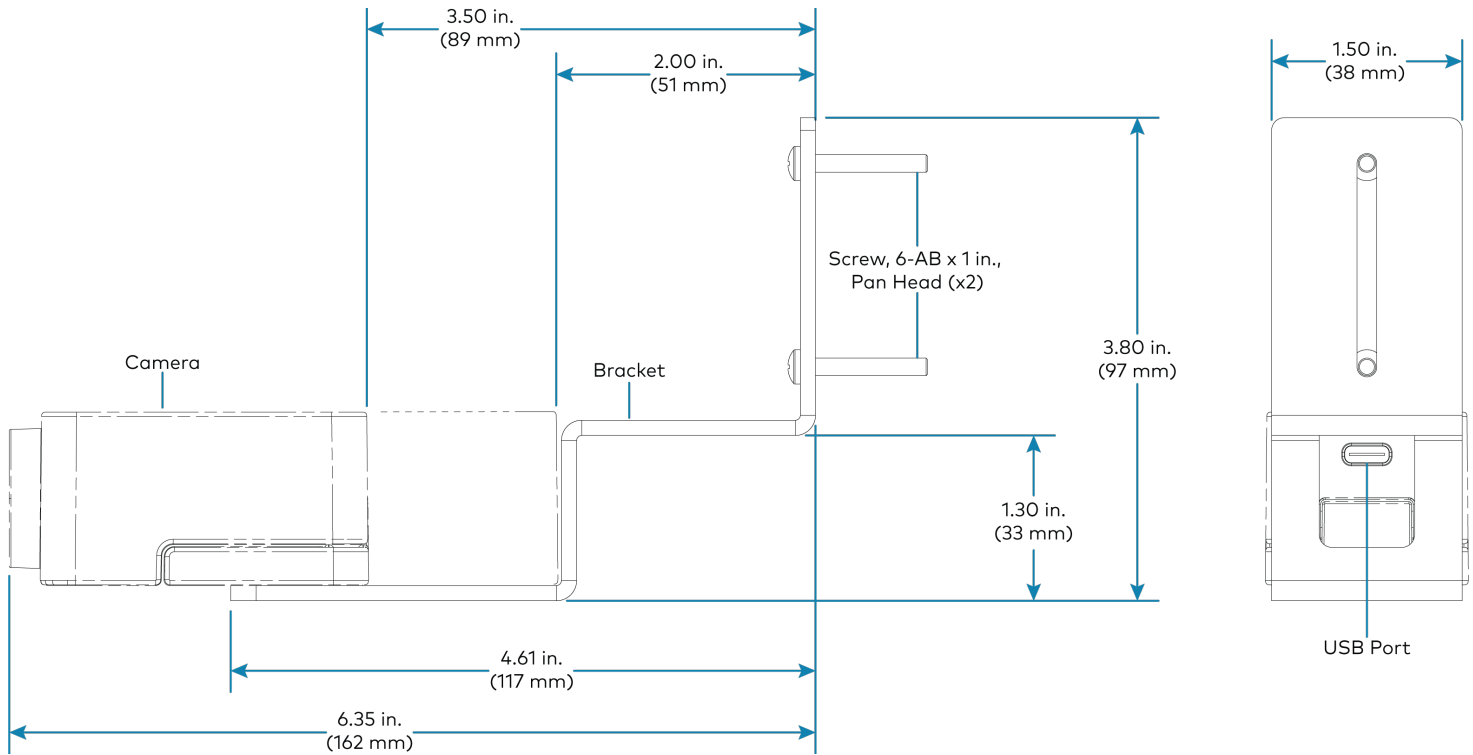
Large Bracket (CCS-CAM-USB-F-400 camera shown)
