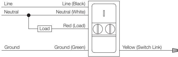
VS 1 Basic Wiring
