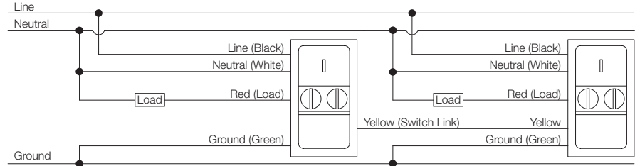
VS 1 (Master / Master) Three-way Wiring - up to maximum 4 sensors can be grouped via "Switch Link"
