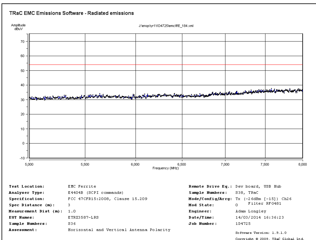
Radiated Transmitter Emissions Channel 26 2480MHz (15.209) Chip Antenna 5GHz-8GHz
