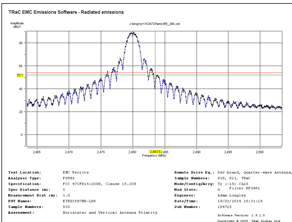
Radiated Transmitter Emissions Channel 26 2480MHz (15.209) Band Edge Compliance Band-Edge plot Quarter-wave Antenna
